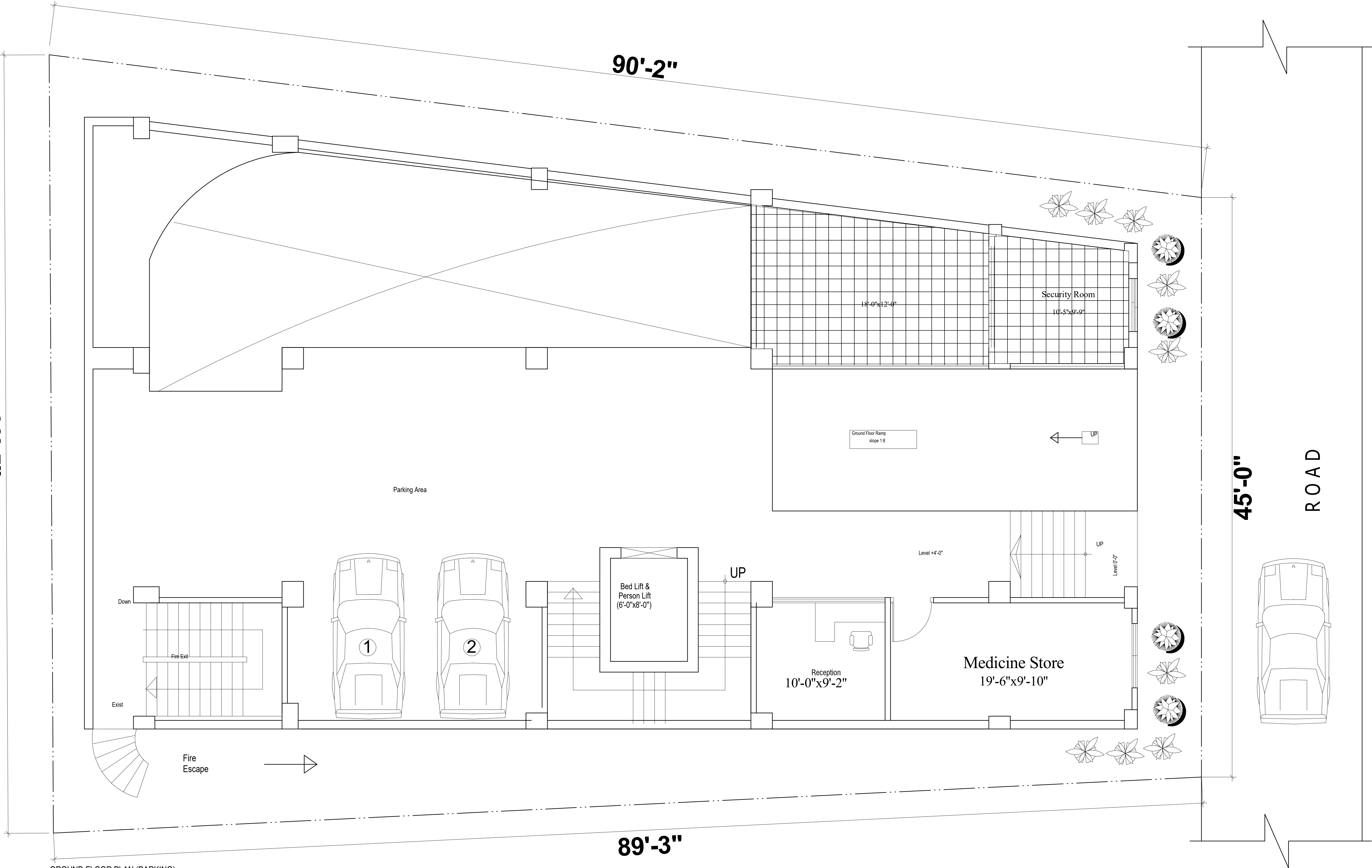
GROUND FLOOR PLAN (PARKING)
