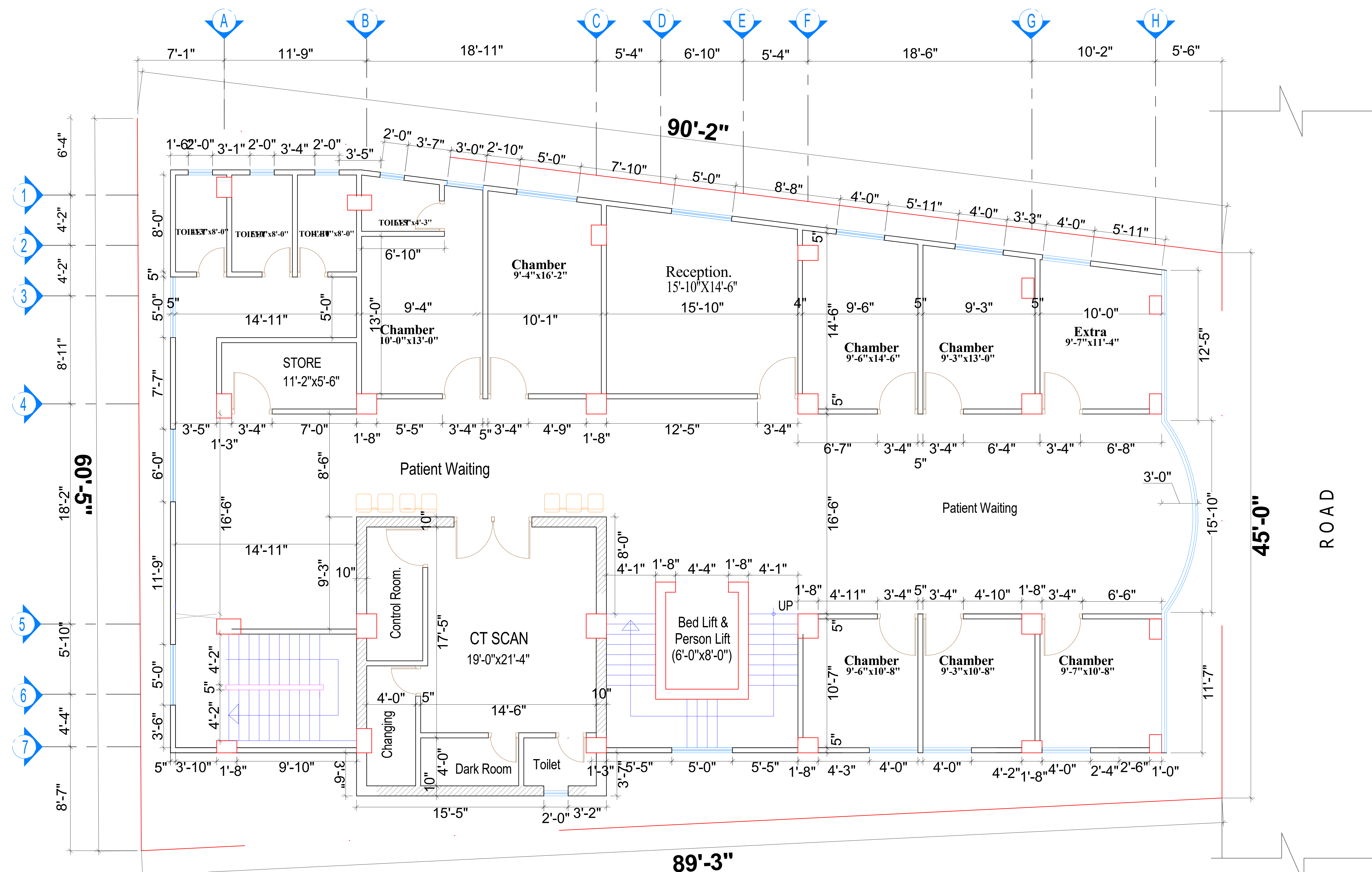
2ND FLOOR PLAN (CONSULTATION+CHAMBER) Floor Area-3658sft
